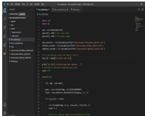
Figure 1: Code snippet for the dataset
