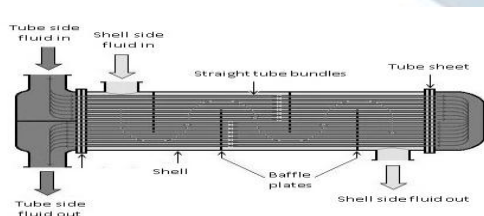
Fig 2: Shell and tube heat exchanger
