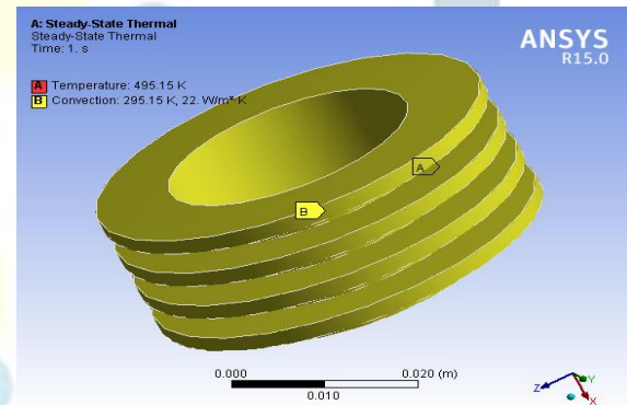
Figure 4: Boundary Conditions
