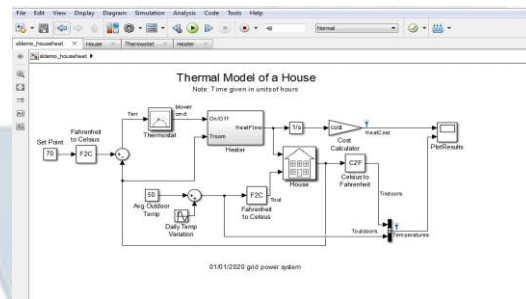
Fig 3: This figure shows Simulation model of a Domestic house.
