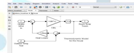
Fig 5: This figure shows the proposed thermostat subsystem.
