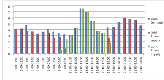
Fig 7: This figure shows the comparative analysis of load demand, grid power supply and \mu grid power supply for 24 hours in Cloudy day.
