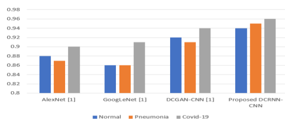
Figure 19: Graphical analysis of precision in Normal, Pneumonia and Covid-19 cases for COVID-19 Chest X-Ray [1] dataset
