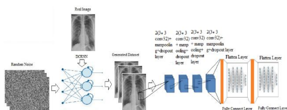
Figure 2: Architecture of proposed CNN+DCRNN model.
