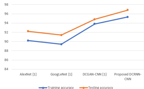
Figure 5: Graphical analysis of training and testing accuracy for COVID-19 X-Ray [1] dataset
