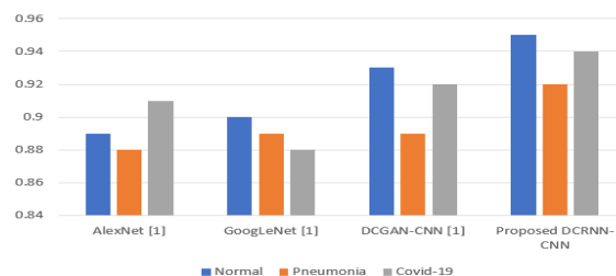
Figure 17: Graphical analysis of precision in Normal, Pneumonia and Covid-19 cases for COVID-19 X-Ray [1] dataset
