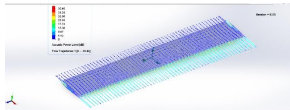
Figure 2: NACA 0012 Blade simulation on Solidworks flow simulation.
