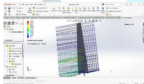
Figure 8: CFD Analysis of Modified wind turbine blade 2 when porous medium is used:
