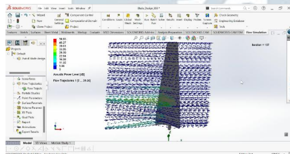
Figure 8: CFD Analysis of Modified wind turbine blade 2 when porous medium is used:
