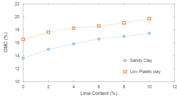
Figure 5: Variation of OMC With Lime Content
