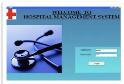
Figure 1: Dialog Box
