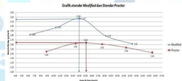
Figure 5: Modified Proctor Compaction Graph Proctor Standard
