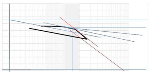
Figure 6: The graph of e \log p
