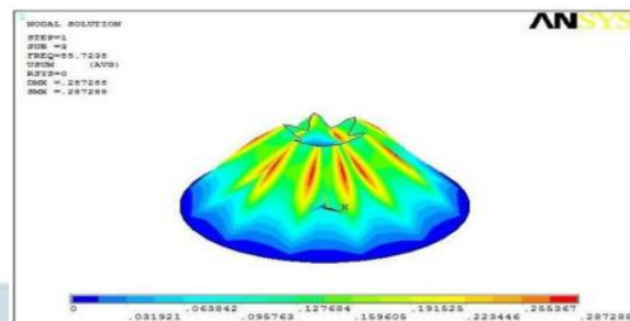
Figure 3: Mode Shapes for Conical Shell (Mode Shape 3-4)
