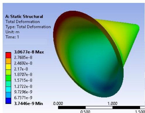
Figure 8: Conical pressure Head total deformation
