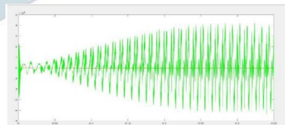
Figure 29: Power outputs from two controls
