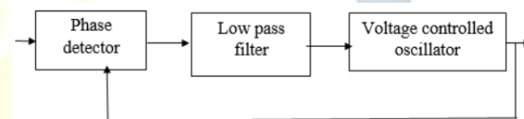
Figure 5: Phase Locked Loop Structure
