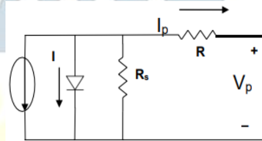
Figure 2: Equivalent Circuit of Solar PV Cell
