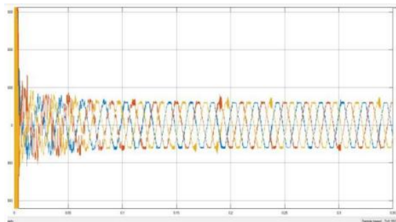
Figure 23: Voltage output from the solar system through inverter
