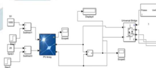
Figure 2: Modeled solar system
