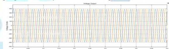
Figure 20: Voltage output from the system with grid dynamics controller having programmable hysteresis switching control
