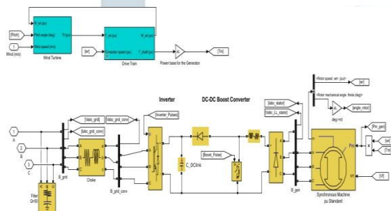
Figure 5: modeled Wind system
