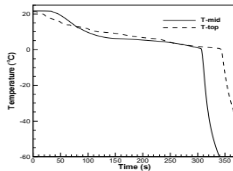
Figure 8: Temperature Variation of PCM in a Cavity of 30 \times 40
