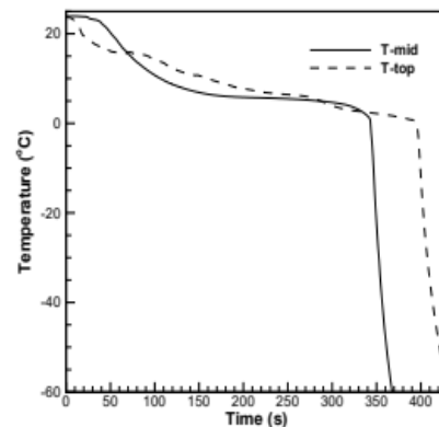
Figure 9: Temperature Variation of PCM in a Cavity of 40 \times 40
