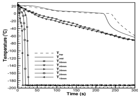
Figure 5: Temperature History for 20 \times 20 Copper Container
