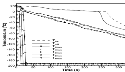
Figure 6: Temperature History for 20 \times 30 Copper Container
