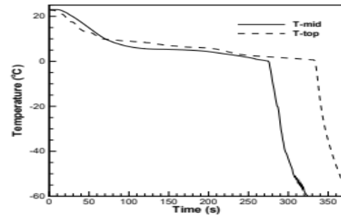
Figure 7: Temperature Variation of The PCM in a Cavity of 30 \times 30
