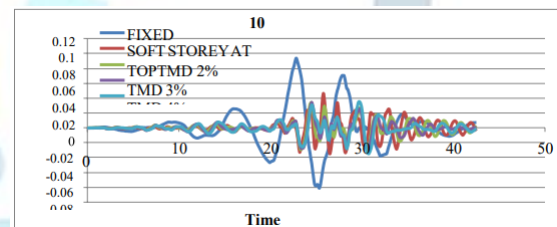
Figure 4.4: Variation of roof displacement for 10 storey model
