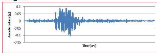
Figure 3.3: Input Time History Acceleration of a Bhuj Earthquake (0.1g)
