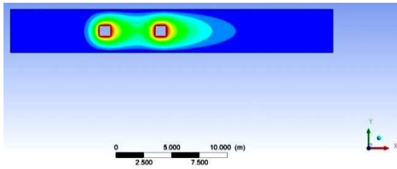
Figure 5: Temperature Profile for Re=50 (Air-Square).
