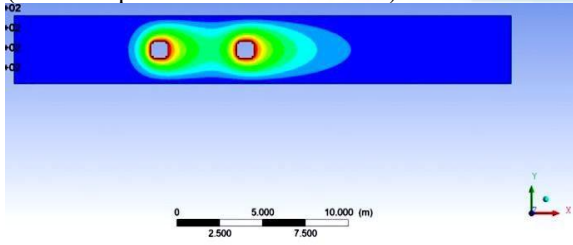
Figure 9: Temperature Profile for Re=50 (Air-Square with square end).
