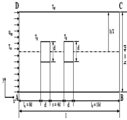
Figure1: Computational domain for square cylinder.
