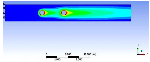
Figure 10: Temperature Profile for Re=50 (Water- Square with square end).
