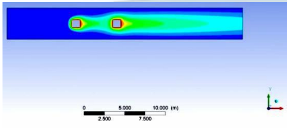
Figure 6: Temperature Profile for Re=50 (Water-Square).
