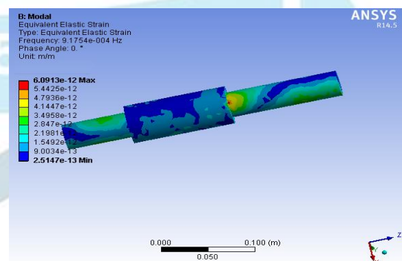
Figure 6: Equivalent elastic strain at 0 degree phase angle.
