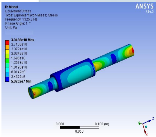
Figure 8: Equivalent Von-mises stress at 1degree phase angle.
