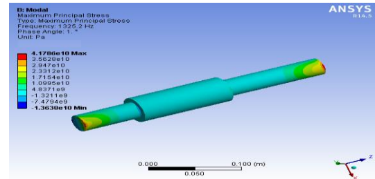
Figure 9: Maximum Principal Stress at 1 degree angle.
