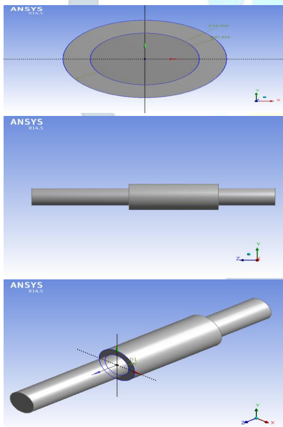
Figure 4: Geometry of shaft in 2D and 3D with dimension in mm.
