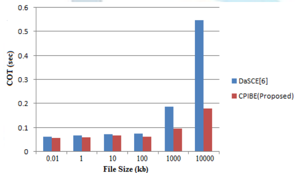
Figure 5: Comparison of Crypto Operation Time (in sec.) in between of DaSCE[6] and CPIBE (Proposed) (download case)
