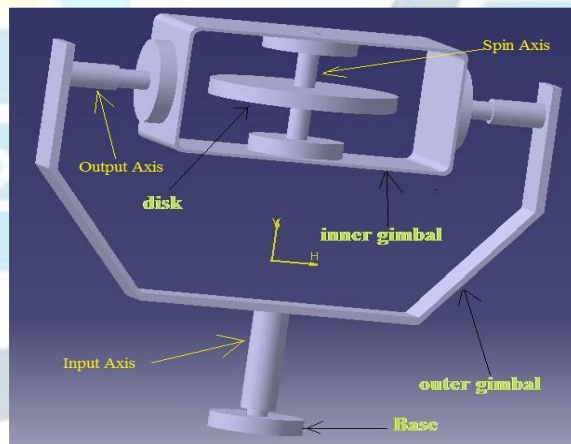
Figure 1: Traditional Gyroscope
