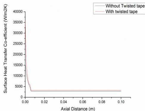
Figure 7: Surface Heat Transfer Coefficient Vs Axial Distance
