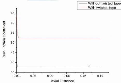
Skin Friction Coefficient
