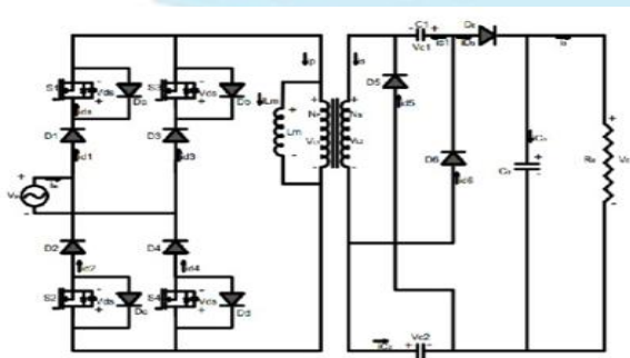
Figure 4: Circuit of Proposed Converter using Switching Capacitor Technique
