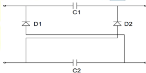
Figure 5: Switched Capacitor Technique
