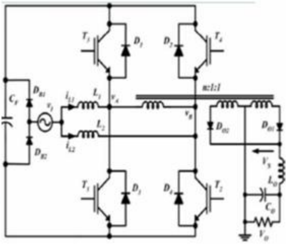
Figure 1: High-efficiency full-bridge single stage topology
