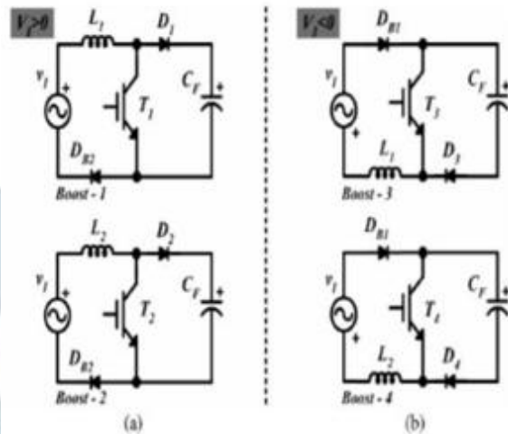
Figure 2: Four boost converters provided by the topology
