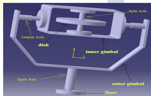
Figure 1: Traditional Gyroscope
