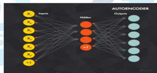
Figure 2: Auto encoders
