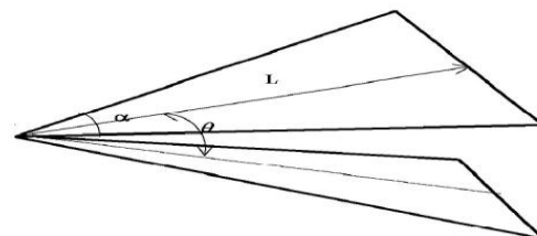
Figure 1: TEM Triangular Antenna
