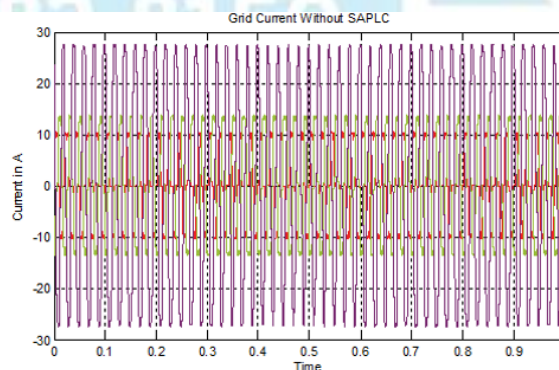
Figure 2: Grid Current without Proposed Work
