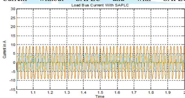
Figure 5: Load Bus Current with SAPLC
