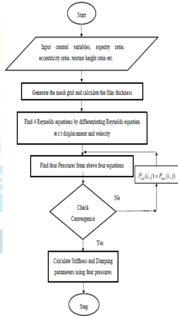
Figure 2: Flow Chart (Dynamic Characteristics)
