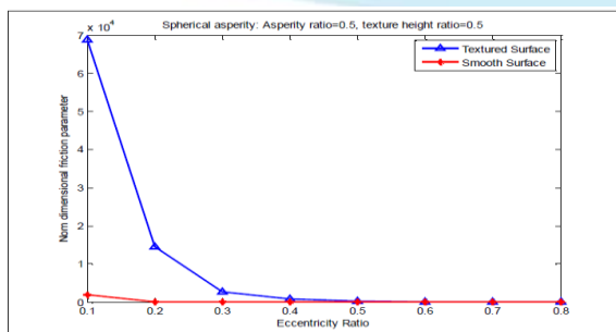
Figure 4: Eccentricity Ratio Vs Friction Parameter
