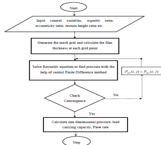
Figure 1: Flow Chart (Static Characteristics)
