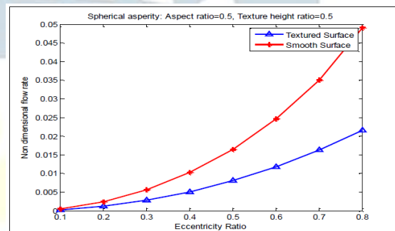
Figure 5: Eccentricity Ratio Vs Non Dimensional Flow Rate
