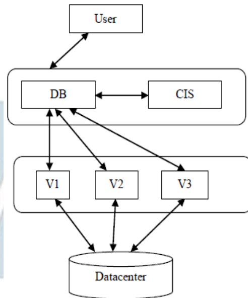
Figure 1: Stages of Scheduling DB: - Datacenter Broker CIS: - Cloud Information administrations V1, V2, V3 are the virtual machines
