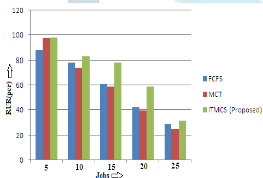
Figure 5: Resource Utilization Rate (sec) among FCFS, MCT and ITMCS
