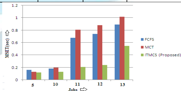
Figure 4: MSET (sec) among FCFS, MCT and ITMCS
