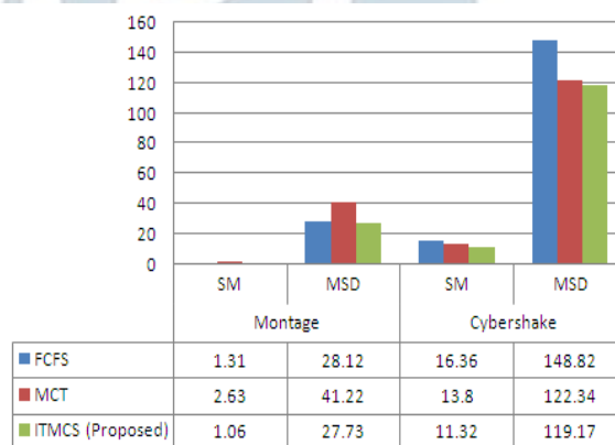
Figure 6: SM and MSD among FCFS, MCT and ITMCS
