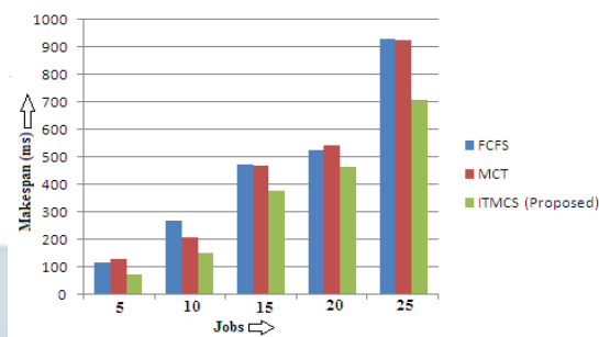
Figure 3: Makespan among FCFS, MCT and ITMCS
