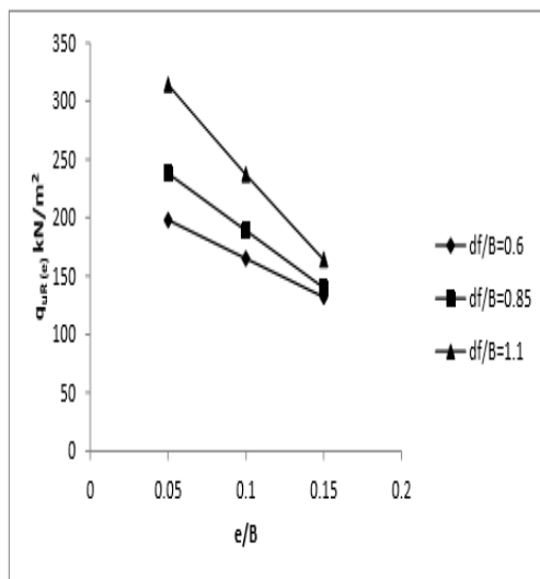
Figure 1: Variation of q_{uR}(e) with e/B for B/L=0.5
