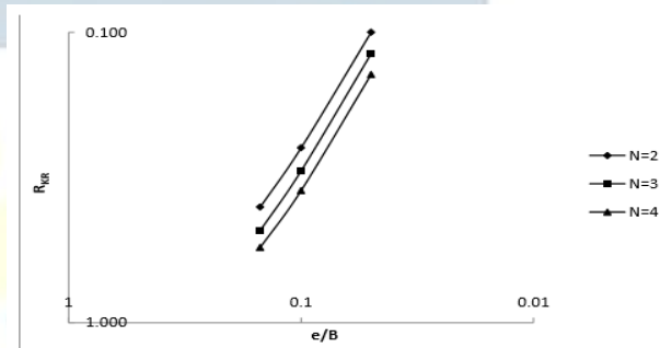
Figure 3: Variation of R_{KR} with e/B for B/L=0.5
