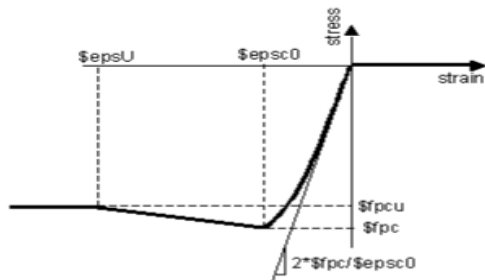
Figure 1: Parameters for OPENSEES
