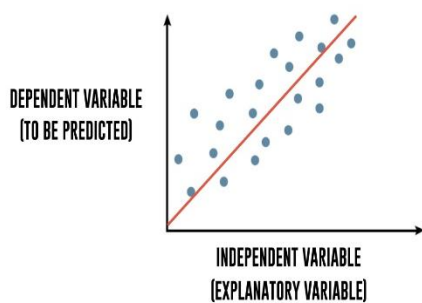
Figure 2: Regression Analysis
