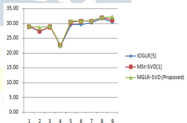
Figure 5: Comparison of PSNR for different methods with \sigma = 50 .
