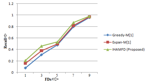
Figure 4: Recall Estimation as per different FDs values (HOSP Dataset)
