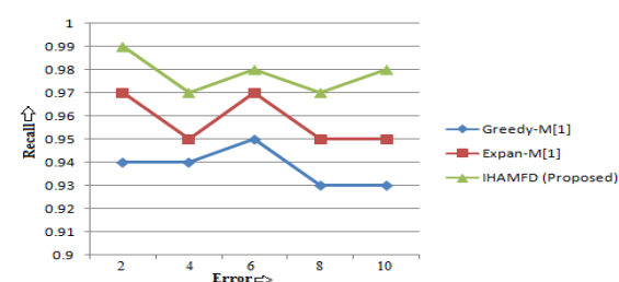
Figure 6: Recall Estimation as per different error rate (HOSP Dataset)
