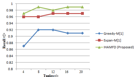
Figure 2: Recall Estimation as per different Tuples values (HOSP Dataset)
