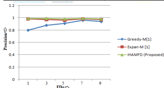
Figure 3: Precision Estimation as per different FDs values (HOSP Dataset)
