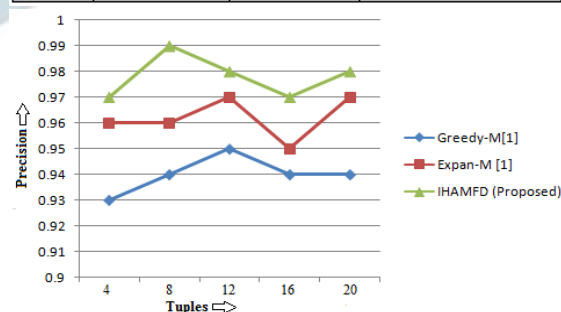
Figure 1: Precision Estimation as per different Tuples values (HOSP Dataset)
