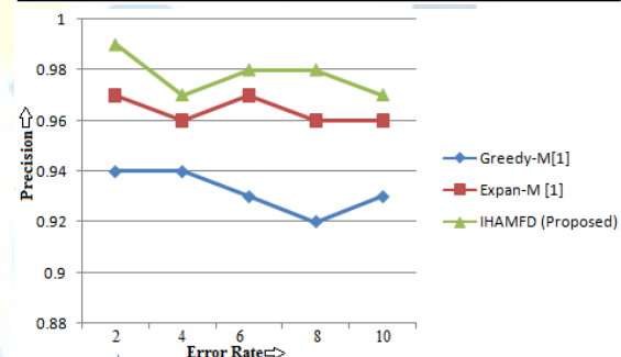
Figure 5: Precision Estimation as per different error rate (HOSP Dataset)
