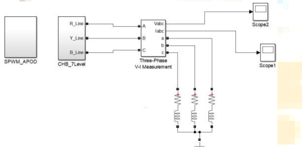
Figure 3: Simulink model of three-phase system with CHB Inverter.
