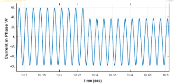
Figure 6: Current waveform of phase A due to short-switch fault in leg 1 of CHB Inverter at t=10.25 sec
