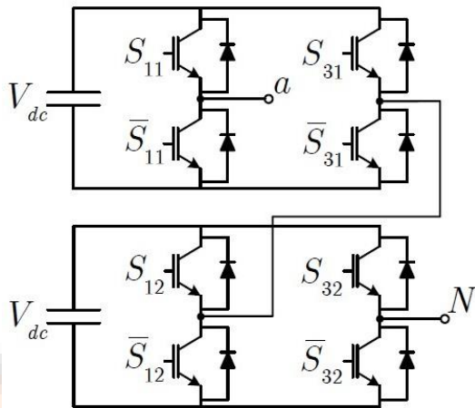
Figure 1: Neutral-point clamped (NPC).
