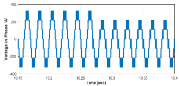
Figure 5: Voltage waveform of phase A due to short-switch fault in leg 1 of CHB Inverter at t=10.25 sec
