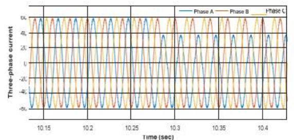
Figure 7: Three-phase Current waveform due to short-switch fault in phase 'A' of CHB Inverter at t=10.25 sec
