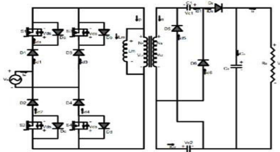
Figure 4: Circuit of Proposed Converter using Switching Capacitor Technique
